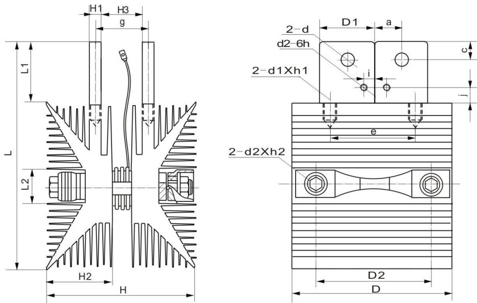
SF11、SF12、SF13 forced air cooling heatsink (with disc device)
