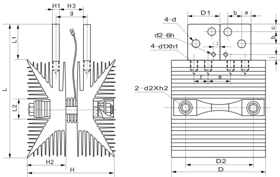
SF14、SF15、SF16、SF17、SF17A、SF18、SF18A forced air cooling heatsink (with disc device)
