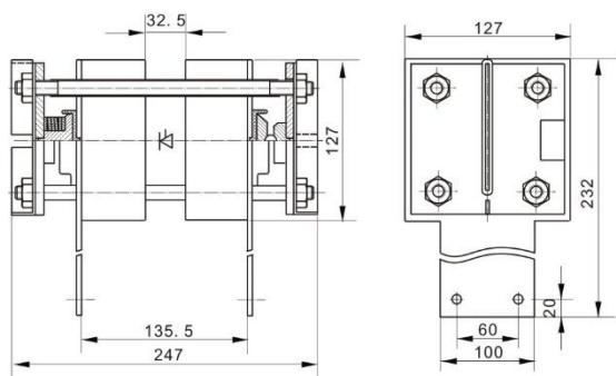
SFA-1 SFA-2 Special air-cooling heatsinks
