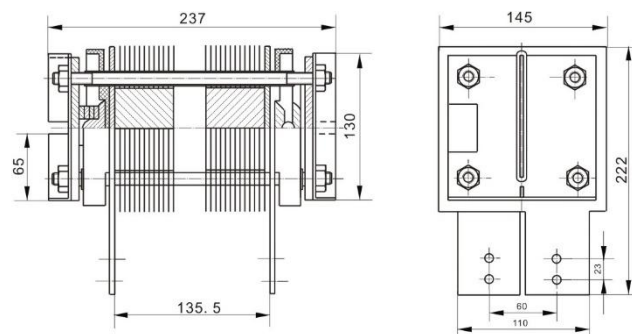
SFA-3 Special air-cooling heatsinks
