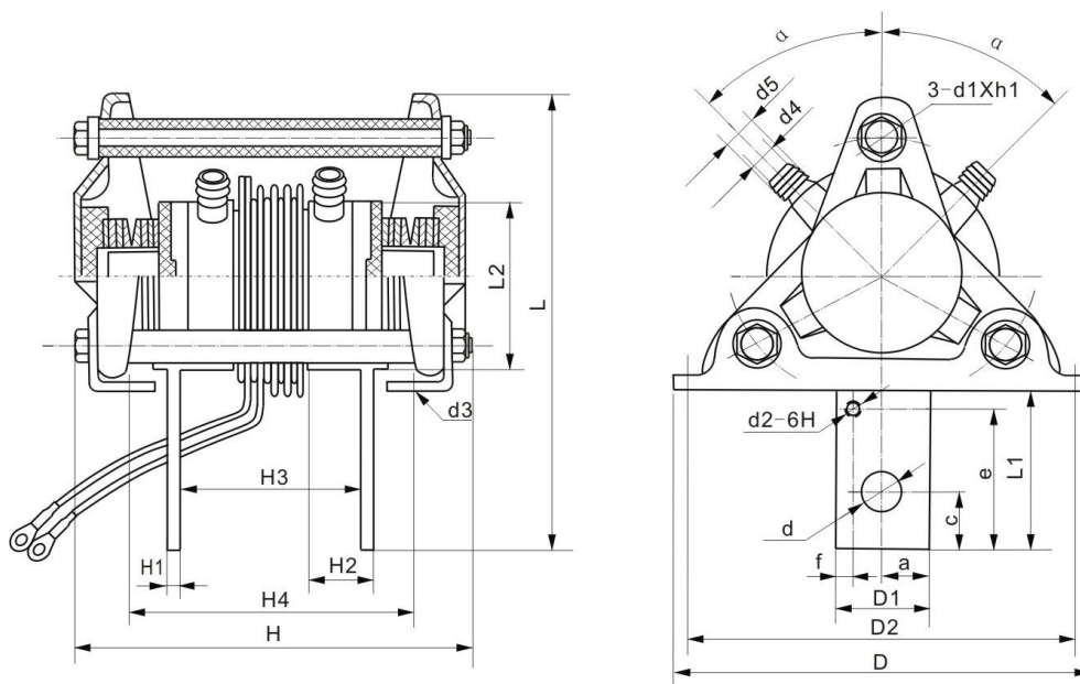
SS11、SS12 water cooling heatsink
