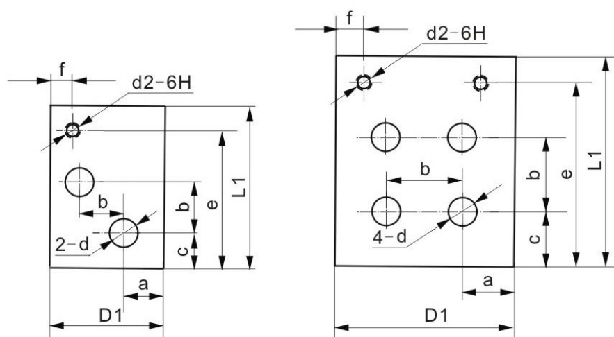
SS13、SS14 conductor plate
